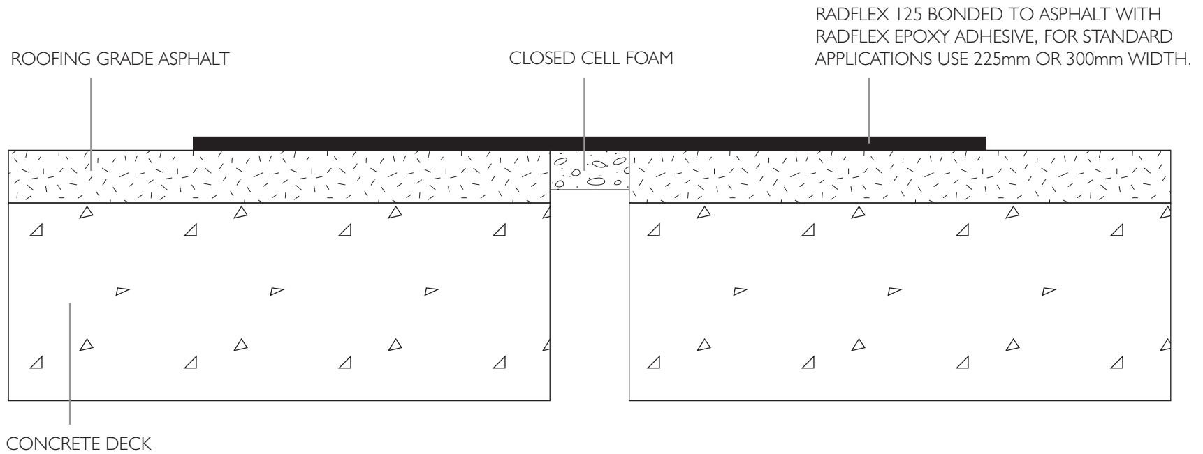
SECTION THROUGH JOINT
