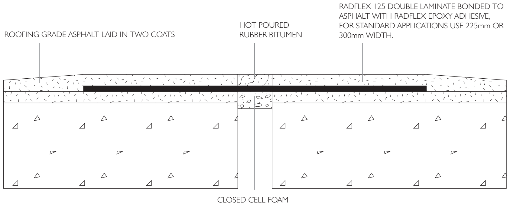
SECTION THROUGH JOINT
